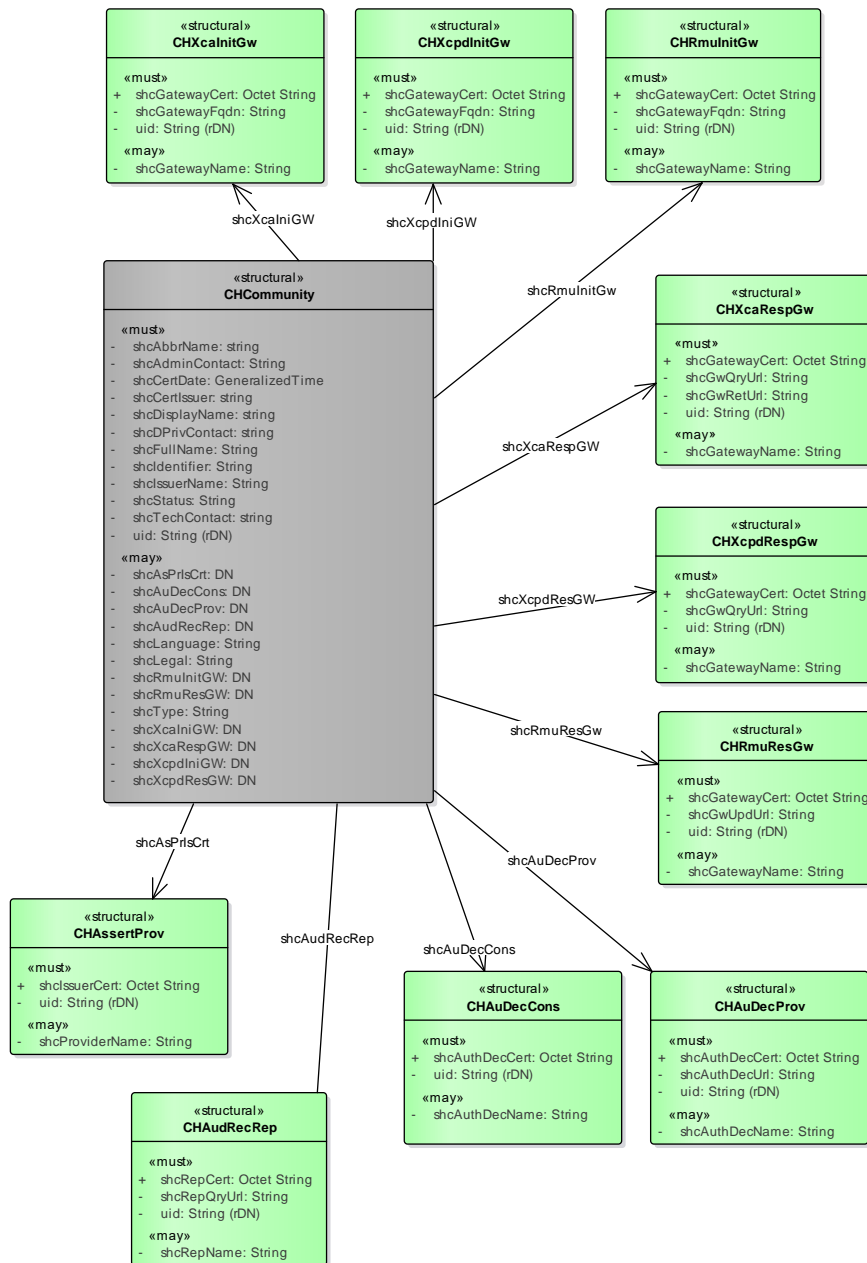
Figure 15: CH:CI LDAP Schema (symbolic representation while incomplete)
