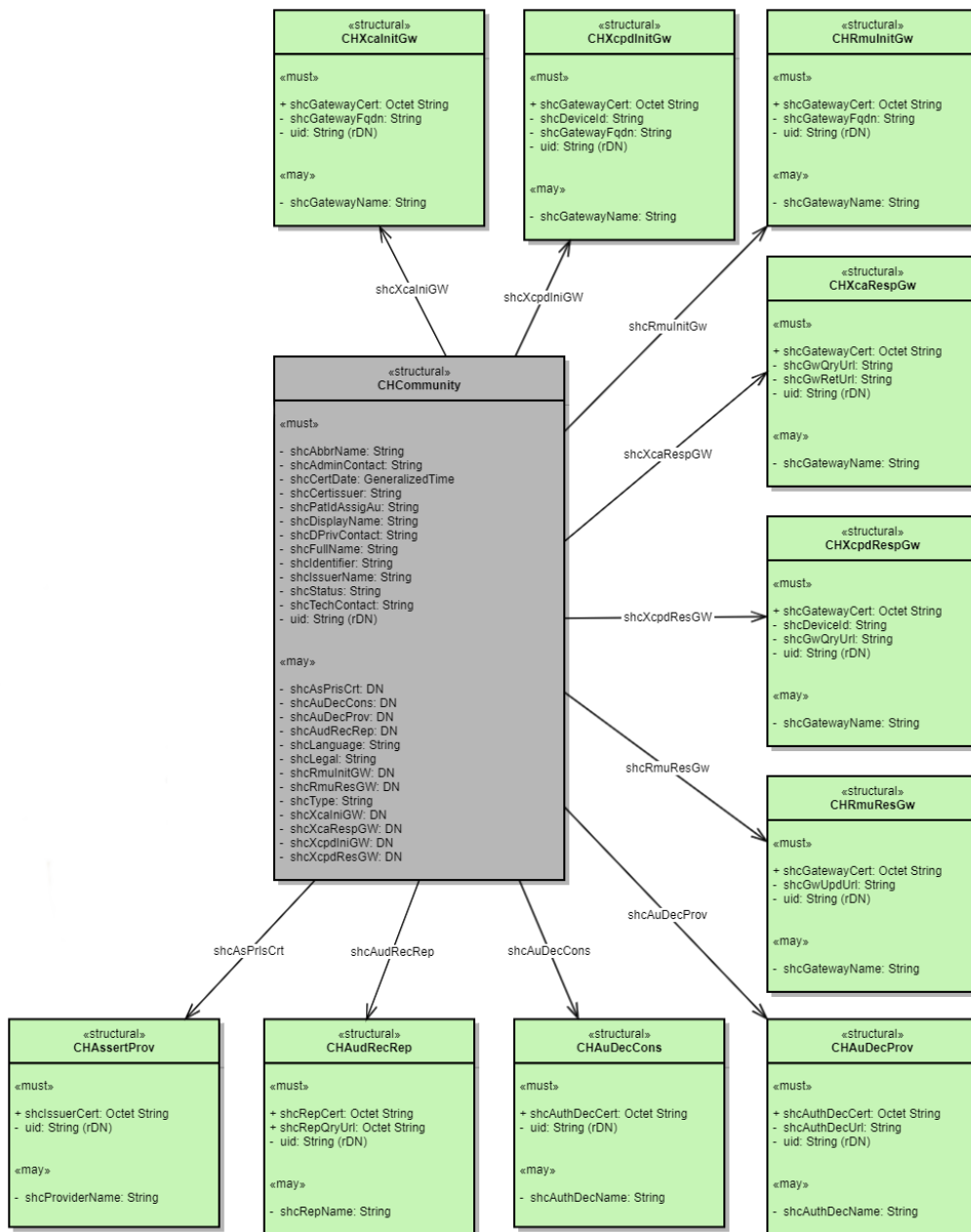
Figure 15: CH:CPI LDAP Schema (symbolic representation while incomplete)
