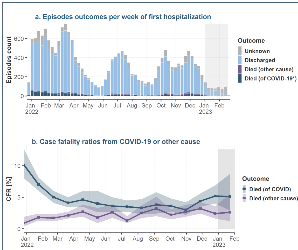
Figure 7: Outcomes for COVID-19 related episodes over time. Includes records up to February 20, 2023. Data from the two last months (highlighted in gray) are considered provisional due to data entry delays. Episodes where the cause of death was not certain, but there was a COVID-19 diagnosis (in conformity with inclusion criteria for CH SUR) were counted as Died of COVID-19 or suspected death of COVID. (* Died of COVID-19 as a confirmed or suspected cause of death). The coloured bands on this plot indicate the 95% confidence interval around the estimated CFR.
