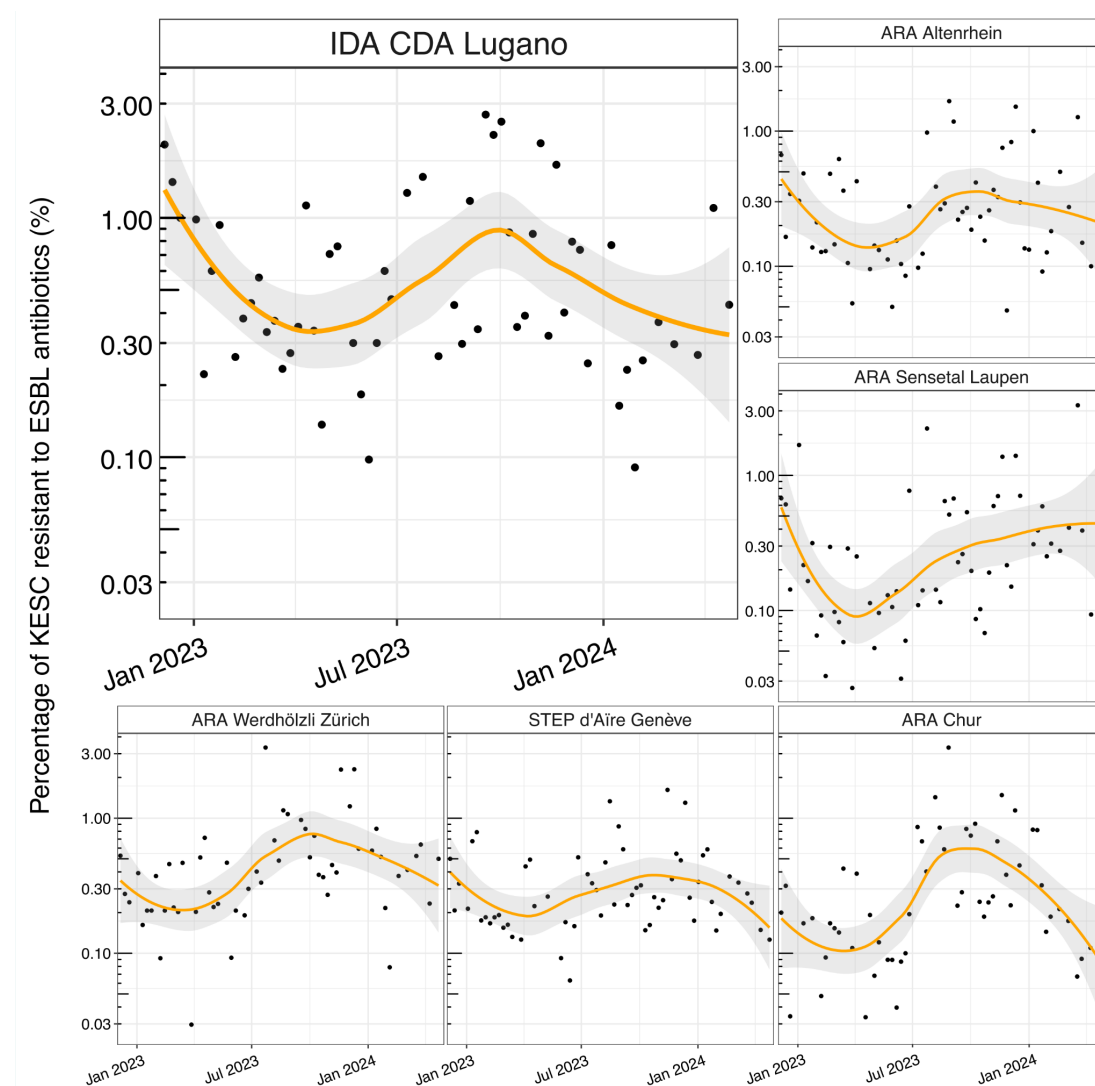
Figure 14: Percentage of extended-spectrum b-lactamase-producing KESC (ESBL-KESC) in wastewater samples from six locations in Switzerland from December 2022 to April 2024. The y-axis is log10 transformed to facilitate visualization of the data. The group KESC refers to the set of microorganisms with similar culturability, including: Klebsiella spp., Enterobacter spp., Citrobacter spp., Serratia spp. Black circles represent measured values, orange line is the LOESS regression, with 95% confidence interval for predictions as grey band.
