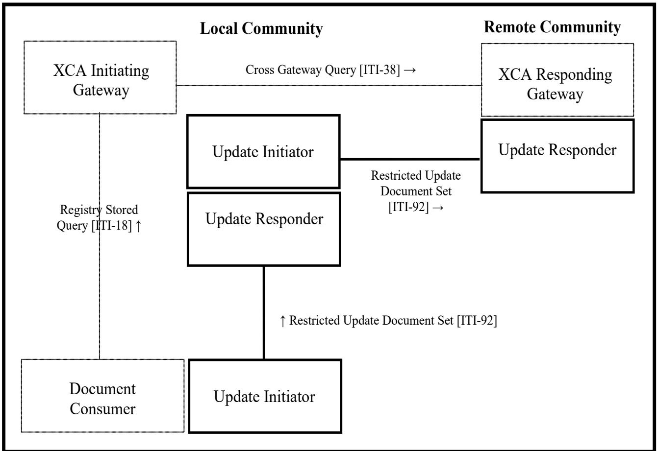
Figure 48.6.3-1: RMU and XCA/XDS Affinity Domain Option Actor Groupings
